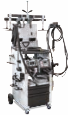
EXPERT 200, 400 + ARCPULL 200, 350
