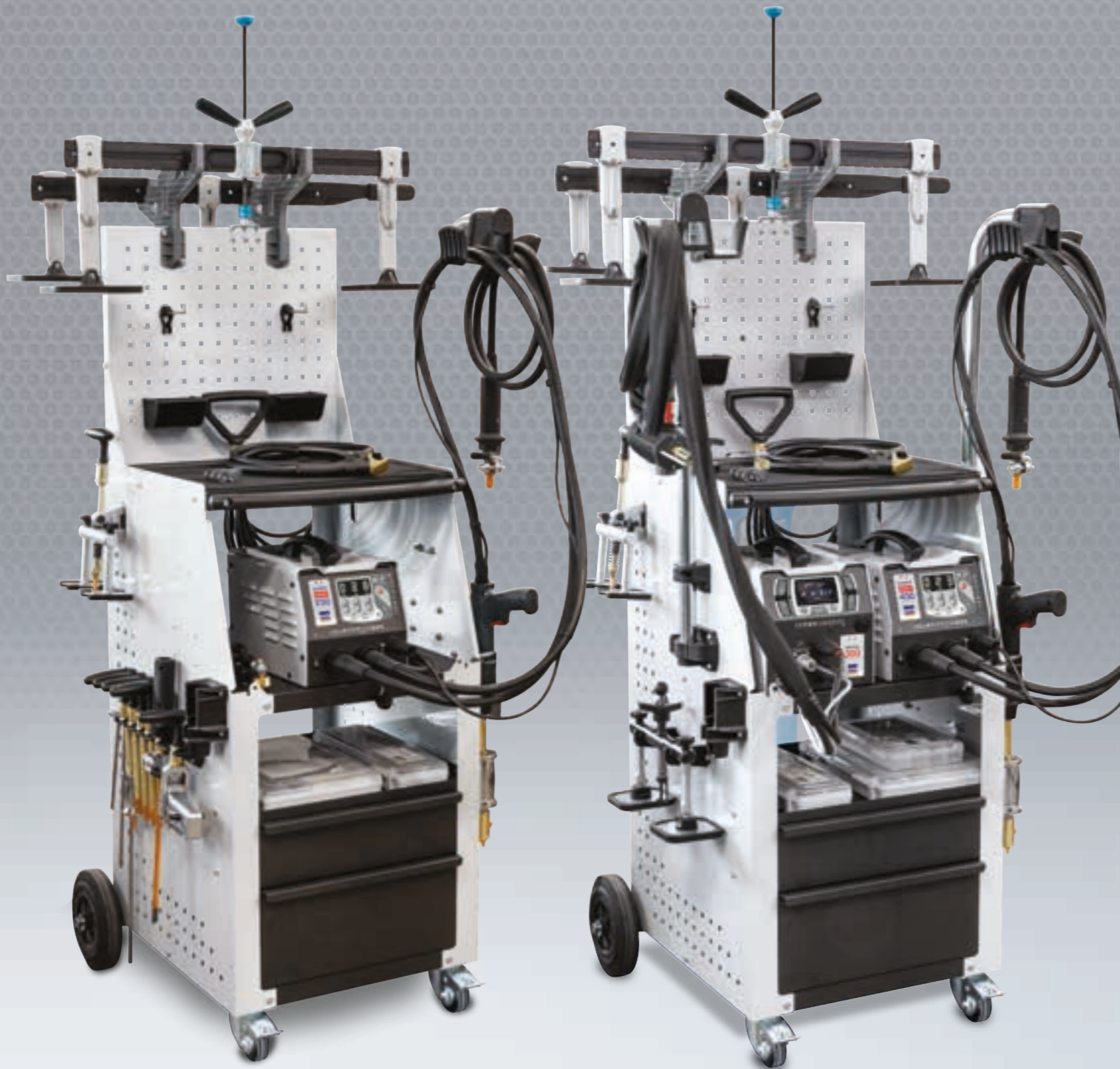
EXPERT 200, 400 + ARCPULL 200, 350
